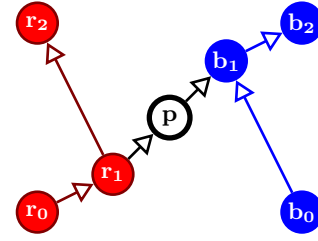
Figure 6: An example system state. The events r_0 , r_1 , and r_2 form transaction R , and the events b_0 , b_1 , and b_2 form transaction B . Event p is not part of either transaction. It may be an input, such as a network delay event, or part of a protocol used to schedule the transactions. In this state, r_1 \rightarrow p \rightarrow b_1 , which means that r_1 happens before b_1 , and so the transactions are ordered: R \rightarrow B .
