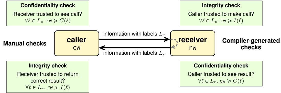
Fig. 7. Manual and compiler-generated checks for remote calls
