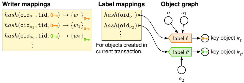
Fig. 16. Writer maps
